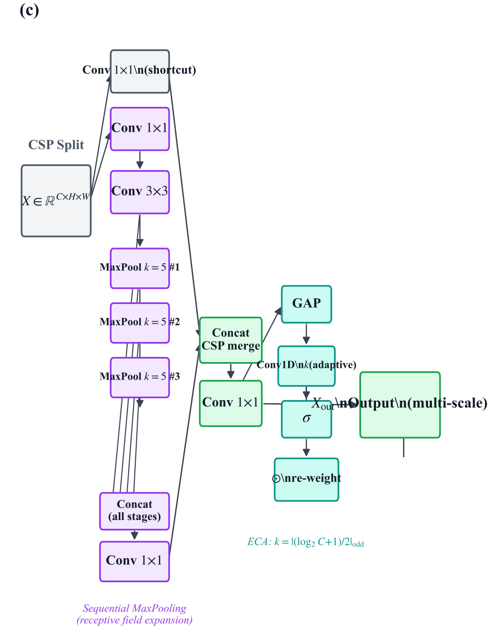
SPPF-CSPC + ECA Module
